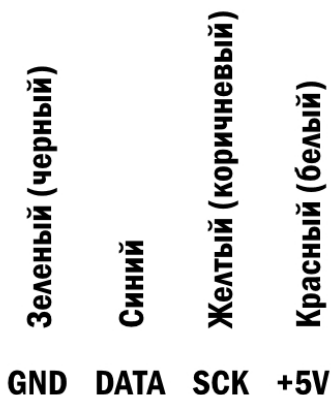
Рис. 9 – Датчики ARHT-01C, ARHT-02C, ARHT-03C, ARHT-04C и ARHT-13C.
